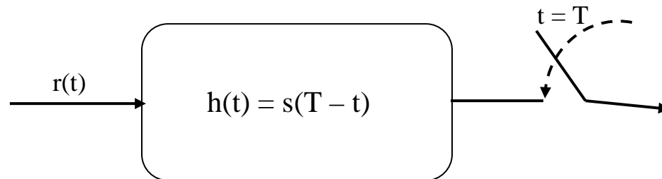
Figure 3.3: Matched filter based spectrum sensing Model for detecting primary users. (Cabric et al.2006)
