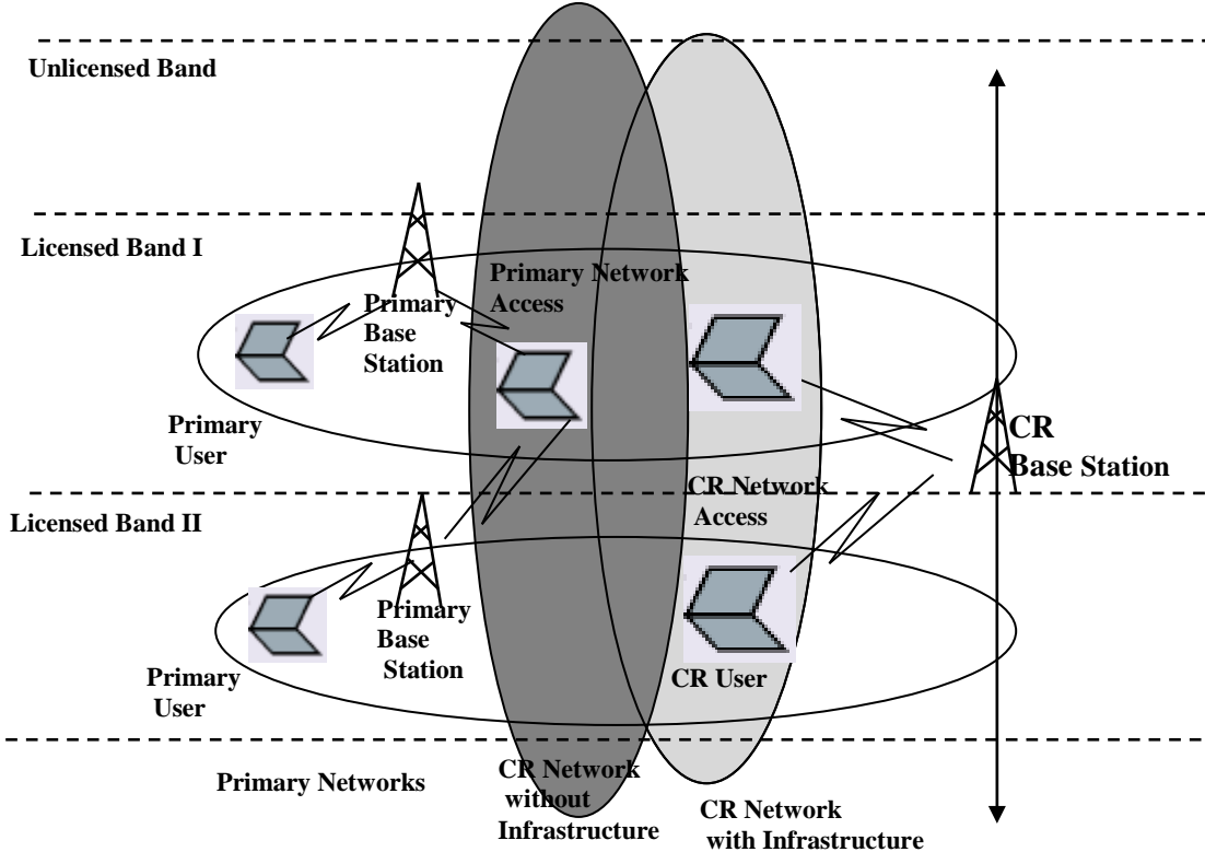
Figure 3.7: Modified Architecture for Cognitive Radio Networks (Source: Rondeau, 2008)
