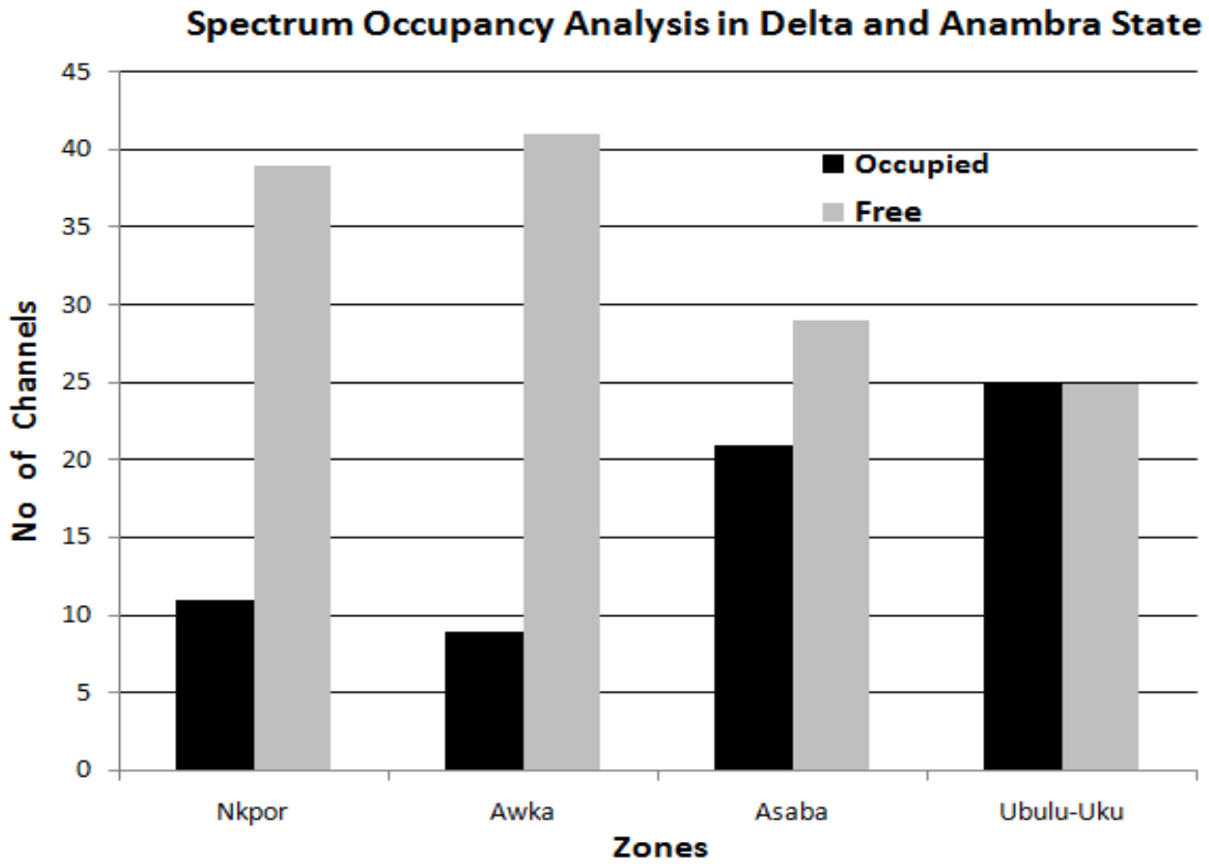
Figure 3.9: Spectrum Occupancy for four Zones
