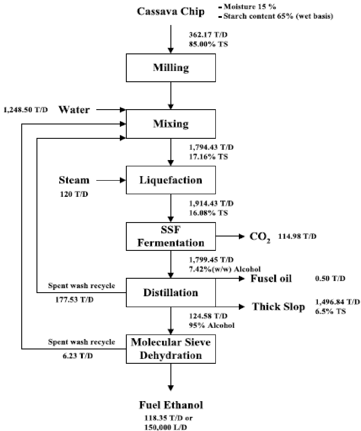
Plate 2: Flow Chart of Ethanol Production from Cassava. Source; (FAO 2000)
